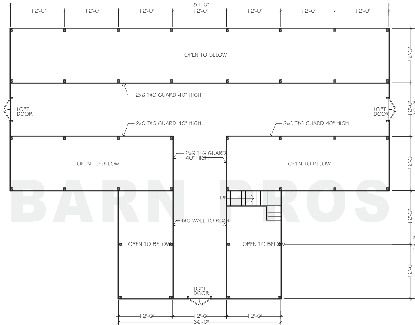
FLOORPLAN - UPPER
