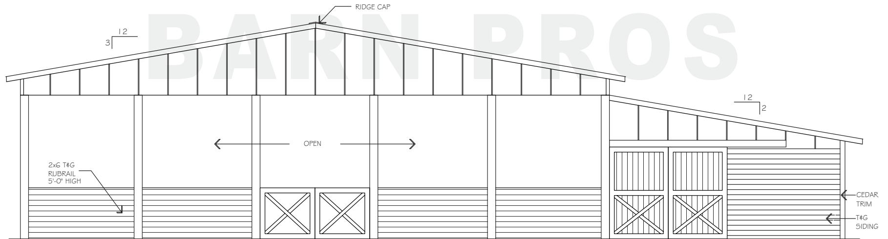
REAR ELEVATION
