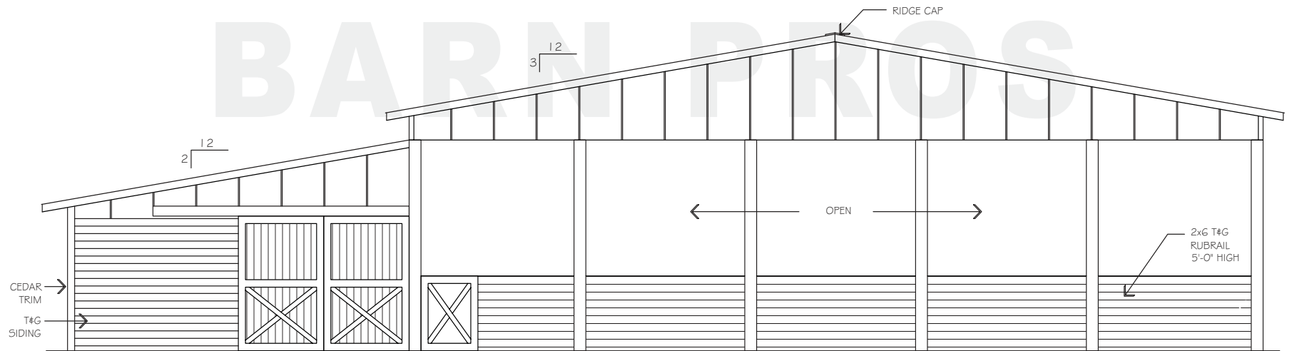
FRONT ELEVATION
