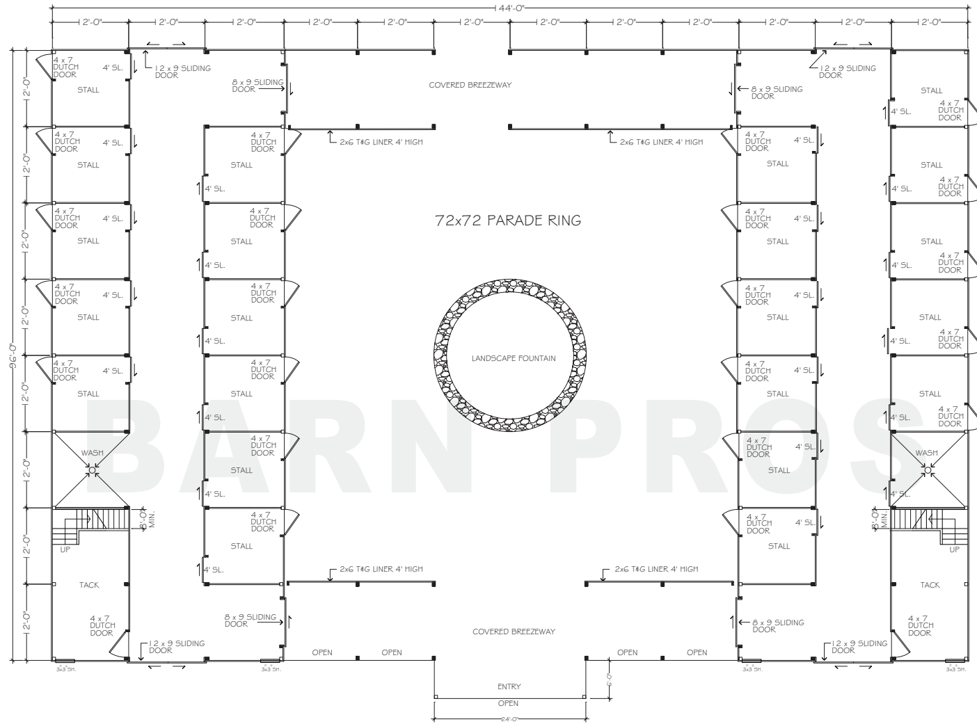
FLOORPLAN - LOWER
