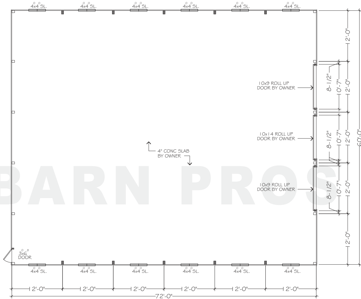
FLOORPLAN - LOWER
