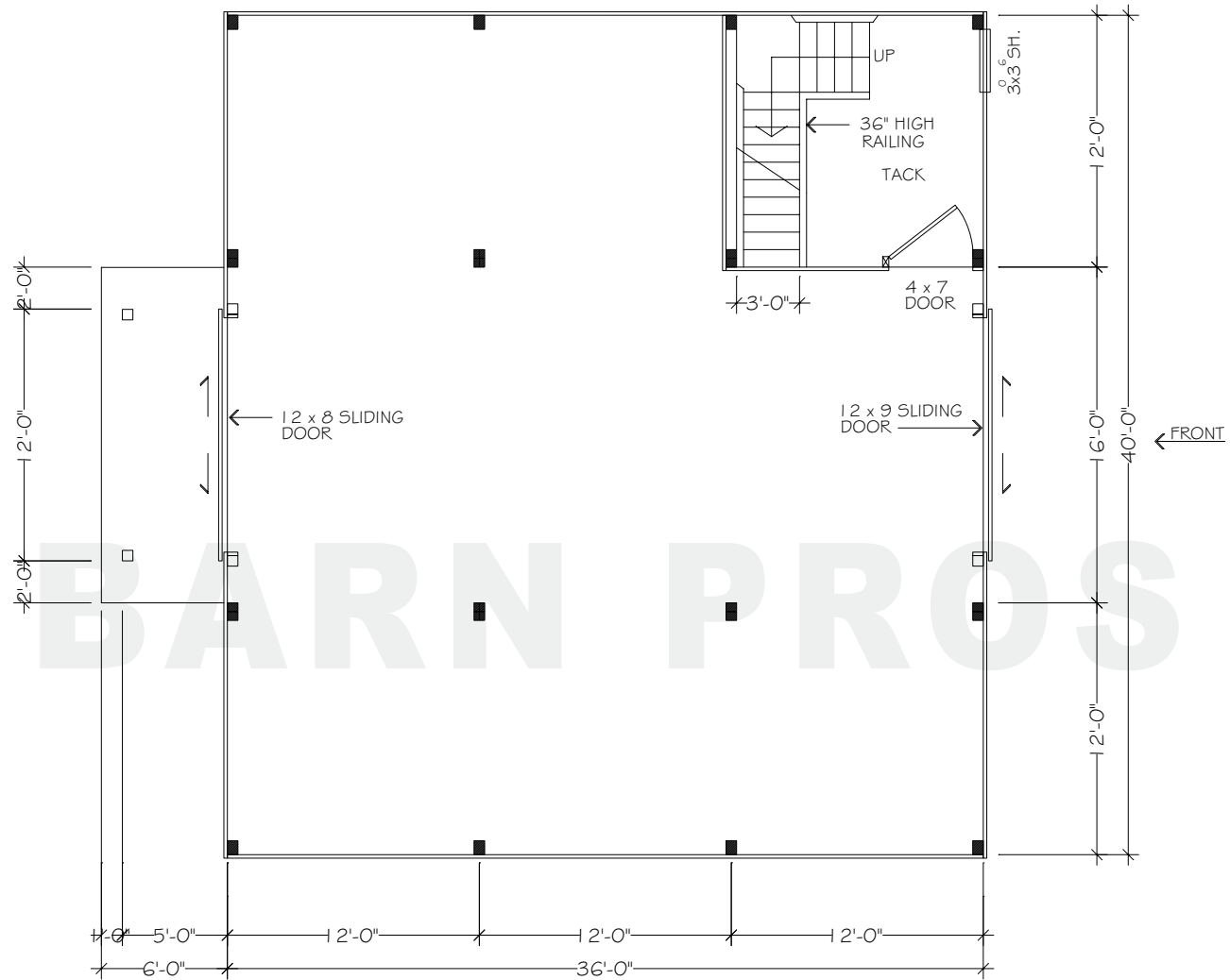
FLOORPLAN - LOWER
