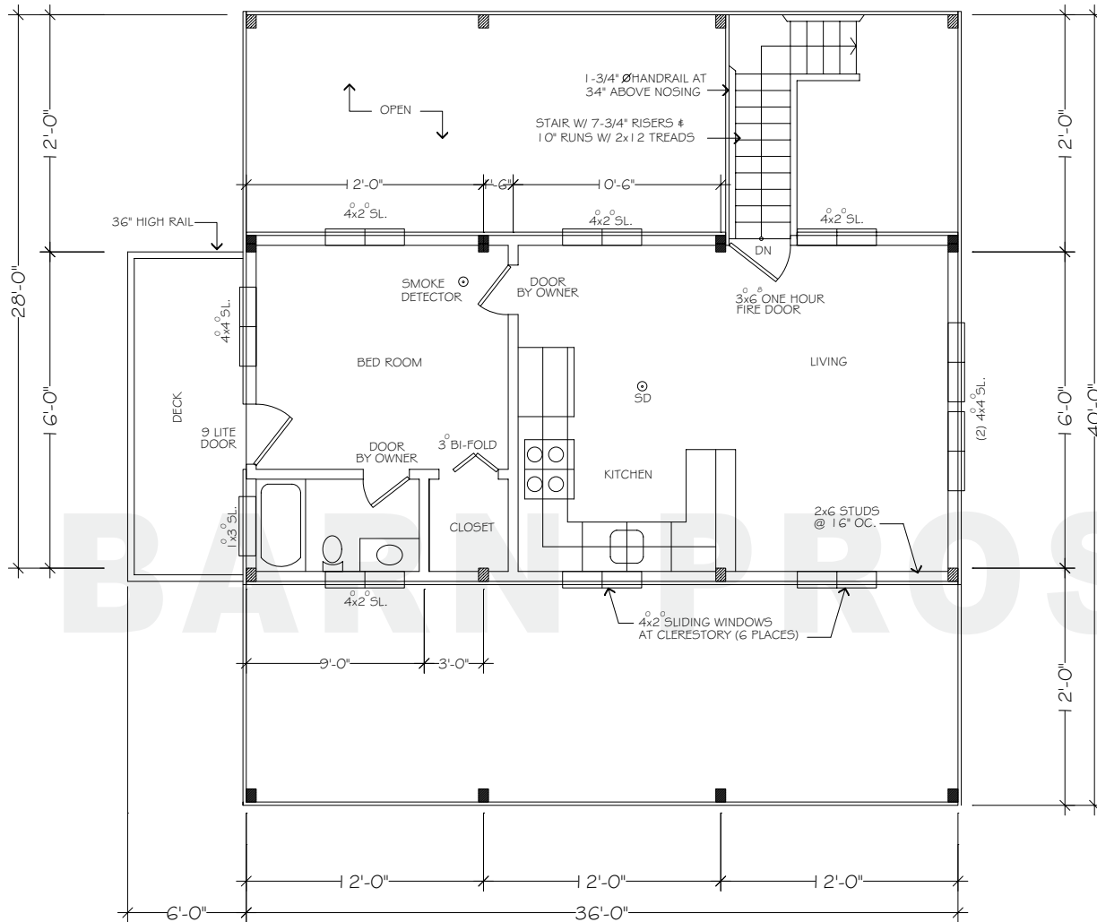
FLOORPLAN - UPPER
