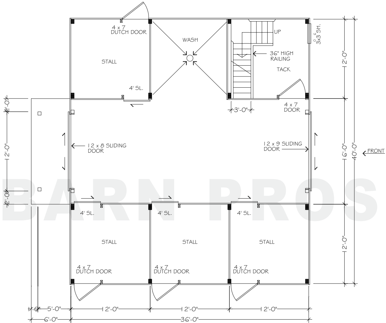
FLOORPLAN - LOWER
