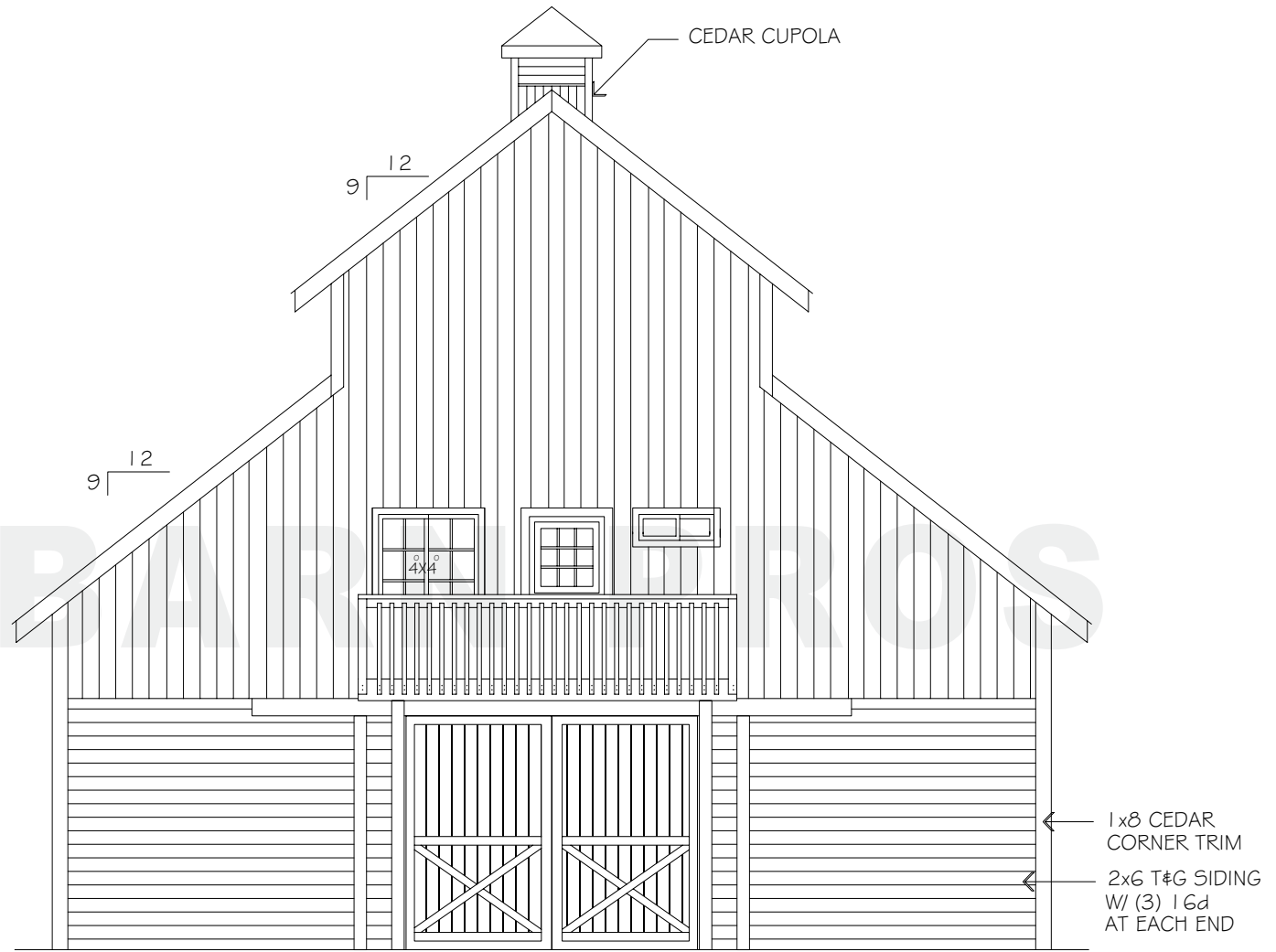
REAR ELEVATION
