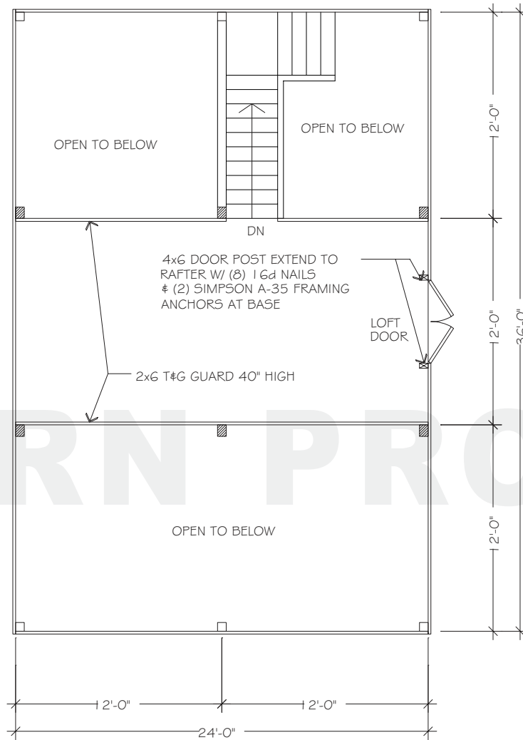
FLOORPLAN - UPPER
