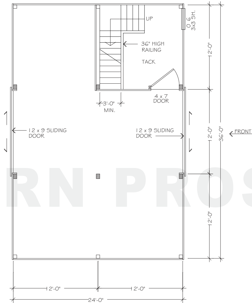
FLOORPLAN - LOWER
