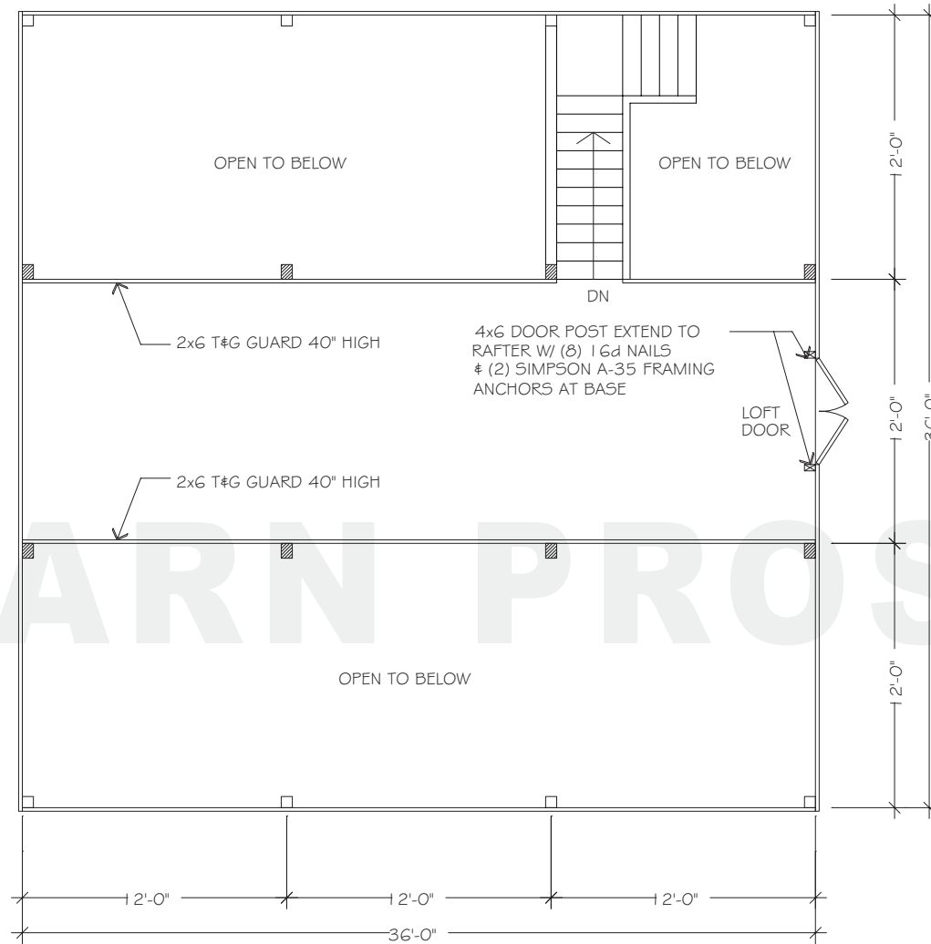
FLOORPLAN - UPPER
