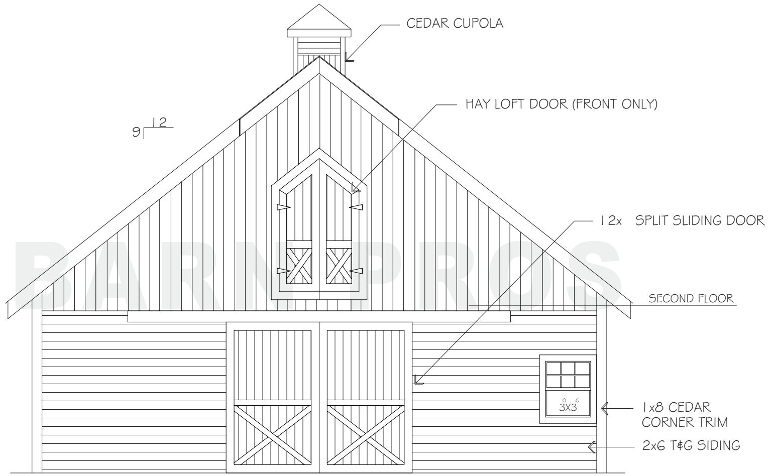
FRONT ELEVATION
