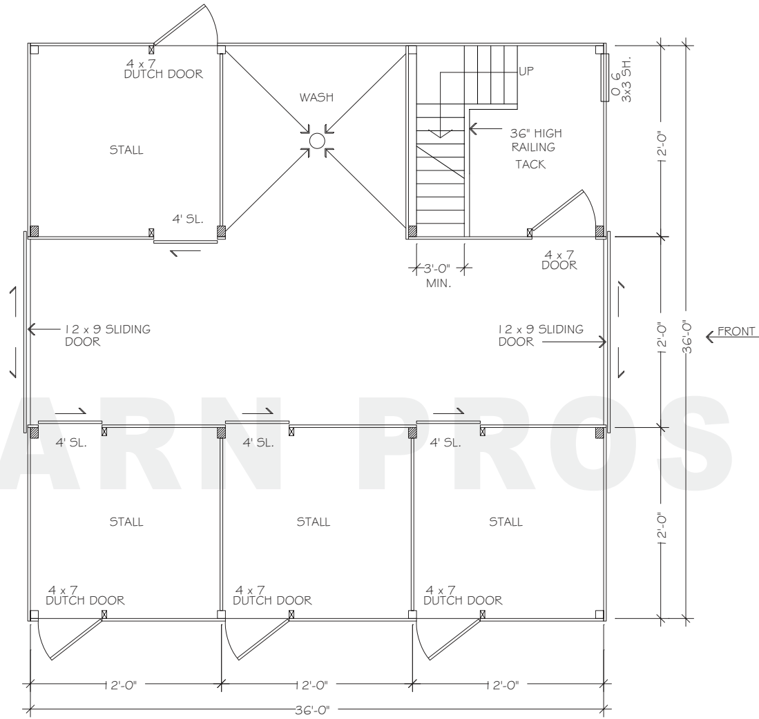
FLOORPLAN - LOWER
