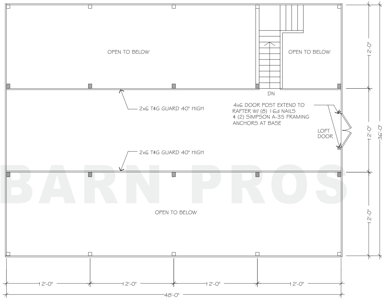
FLOORPLAN - UPPER
