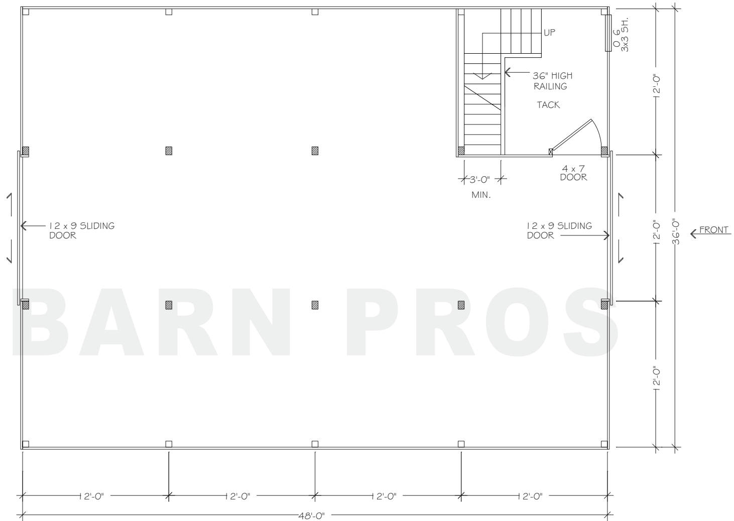
FLOORPLAN - LOWER
