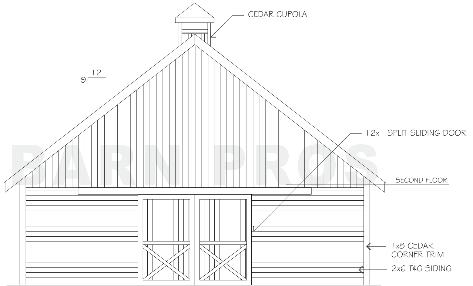
REAR ELEVATION
