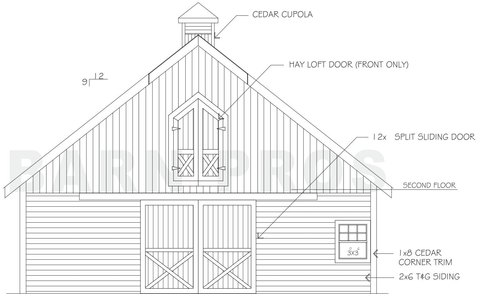
FRONT ELEVATION
