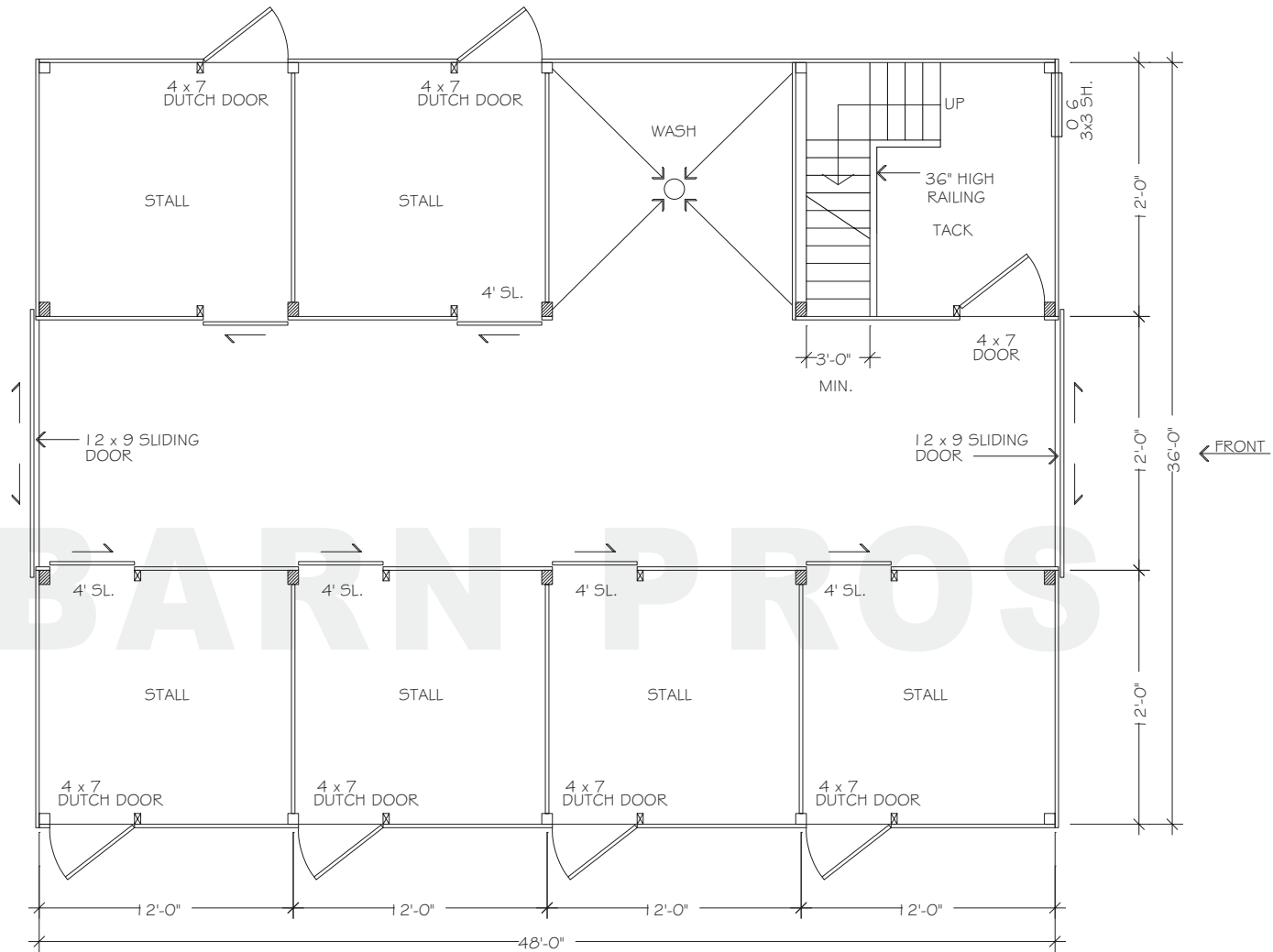
FLOORPLAN - LOWER
