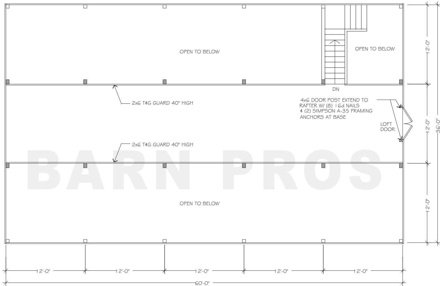
FLOORPLAN - UPPER
