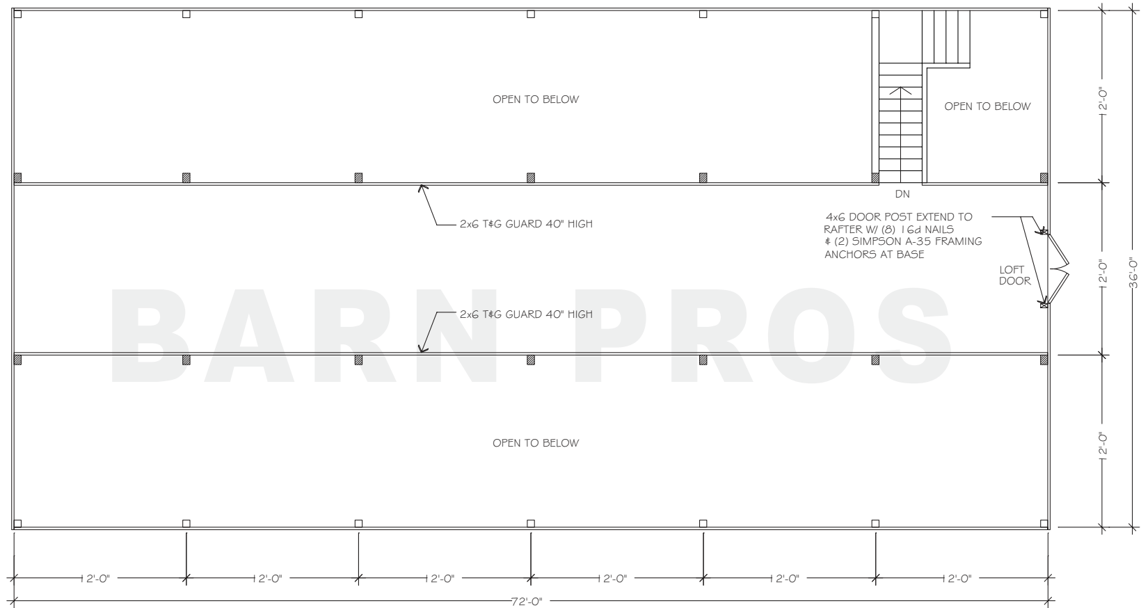
FLOORPLAN - UPPER
