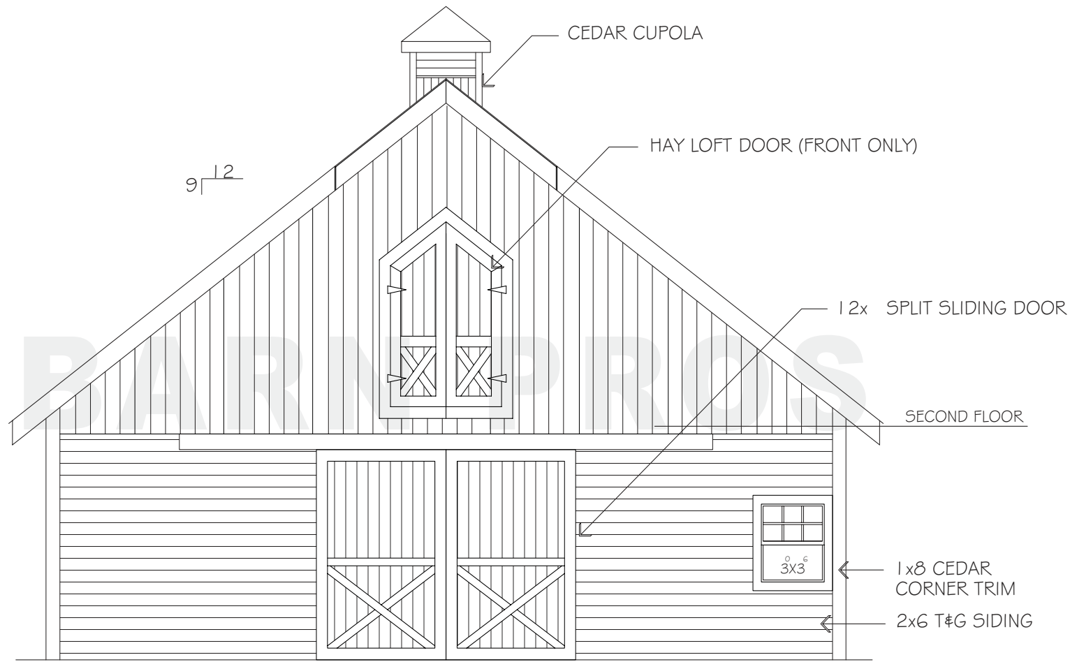
FRONT ELEVATION
