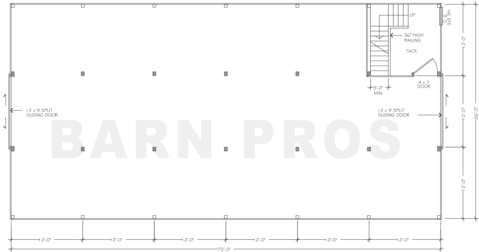
FLOORPLAN - LOWER
