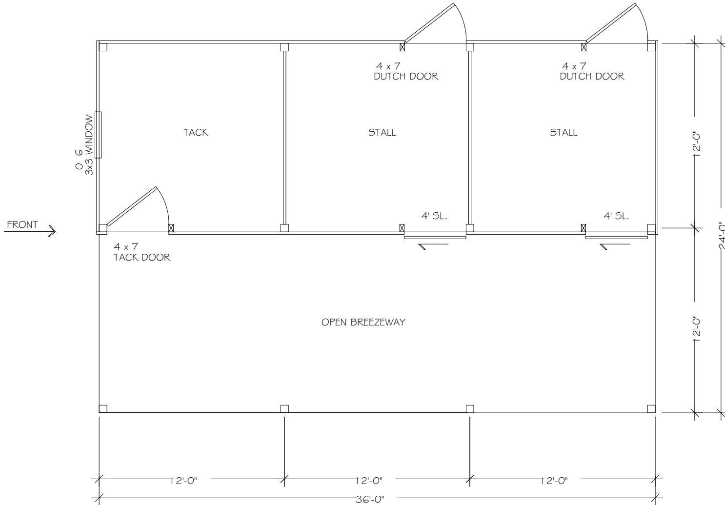
FLOORPLAN
