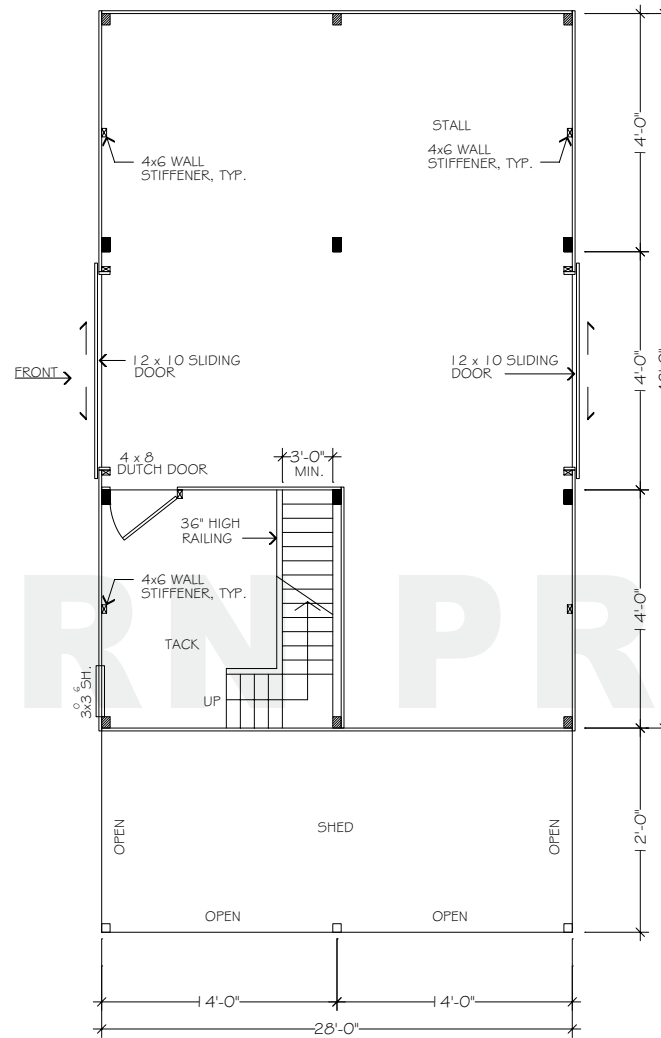
FLOORPLAN - LOWER
