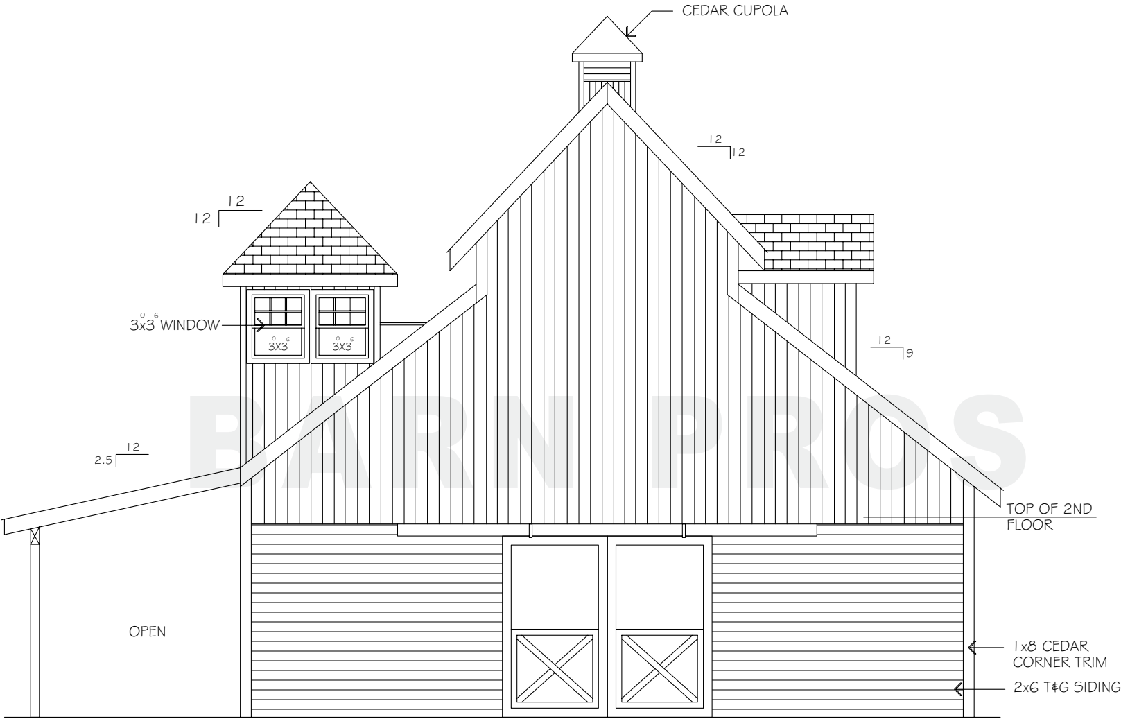
REAR ELEVATION
