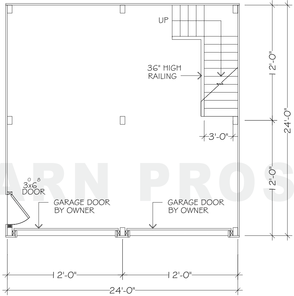
FLOORPLAN - LOWER
