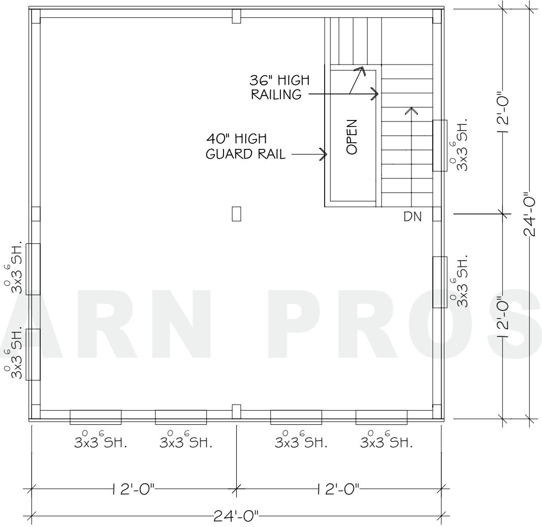
FLOORPLAN - UPPER
