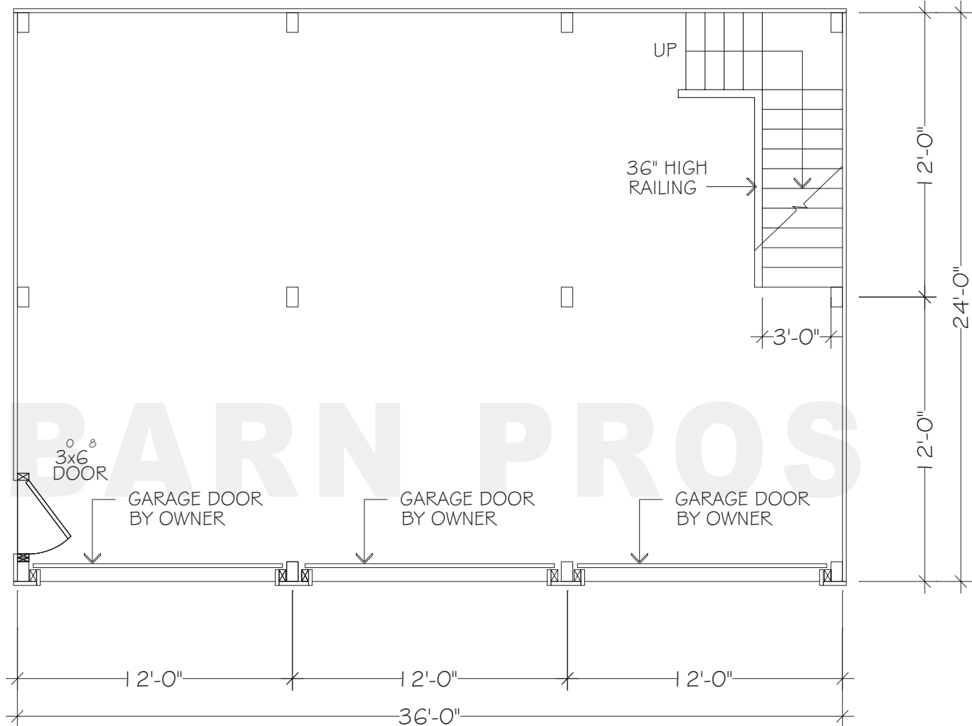
FLOORPLAN - LOWER
