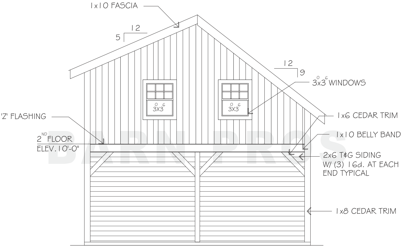
REAR ELEVATION
