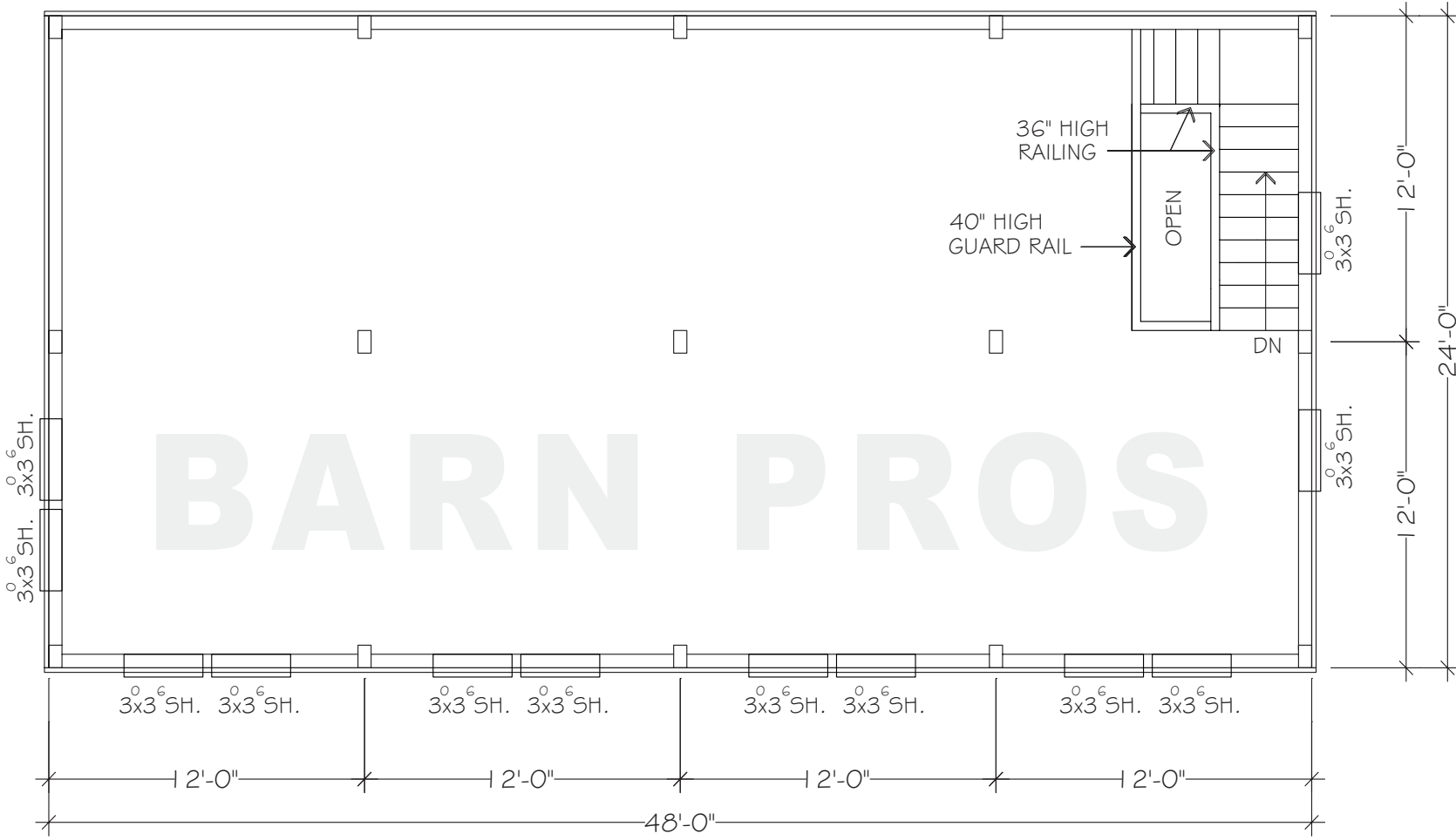
FLOORPLAN - UPPER
