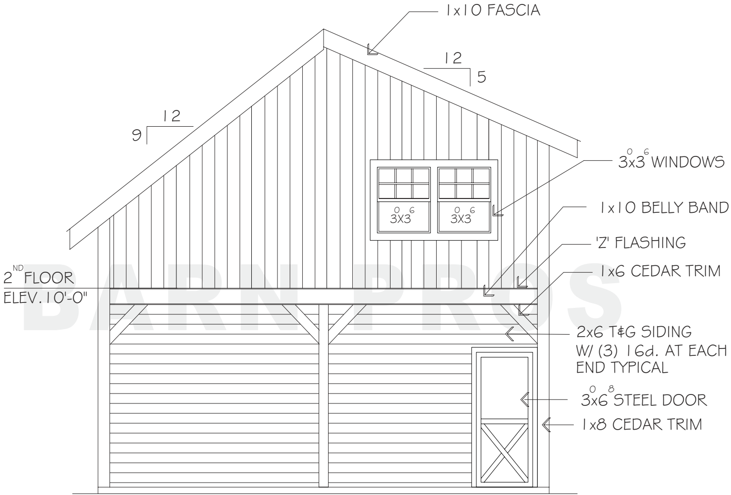
FRONT ELEVATION
