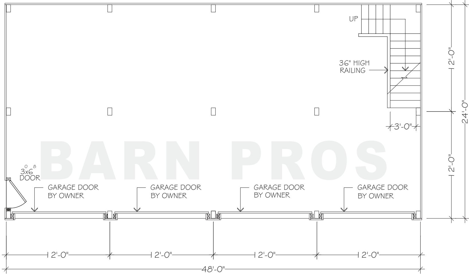
FLOORPLAN - LOWER
