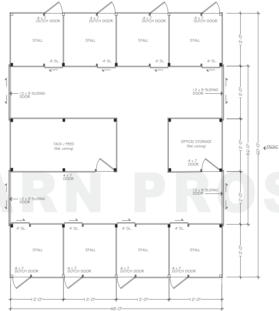
FLOORPLAN - LOWER
