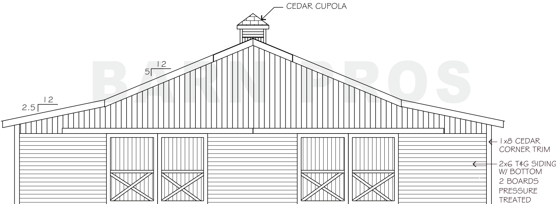
FRONT ELEVATION
