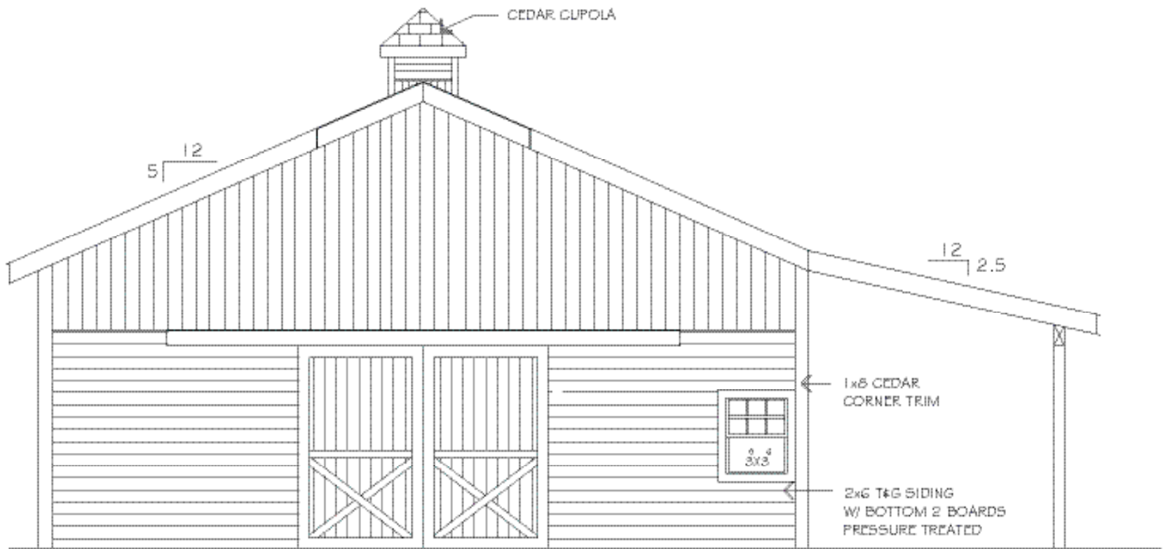
FRONT ELEVATION
