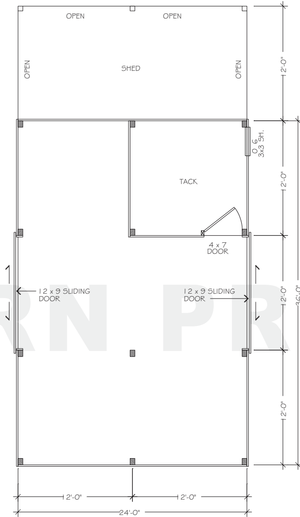
FLOORPLAN - LOWER
