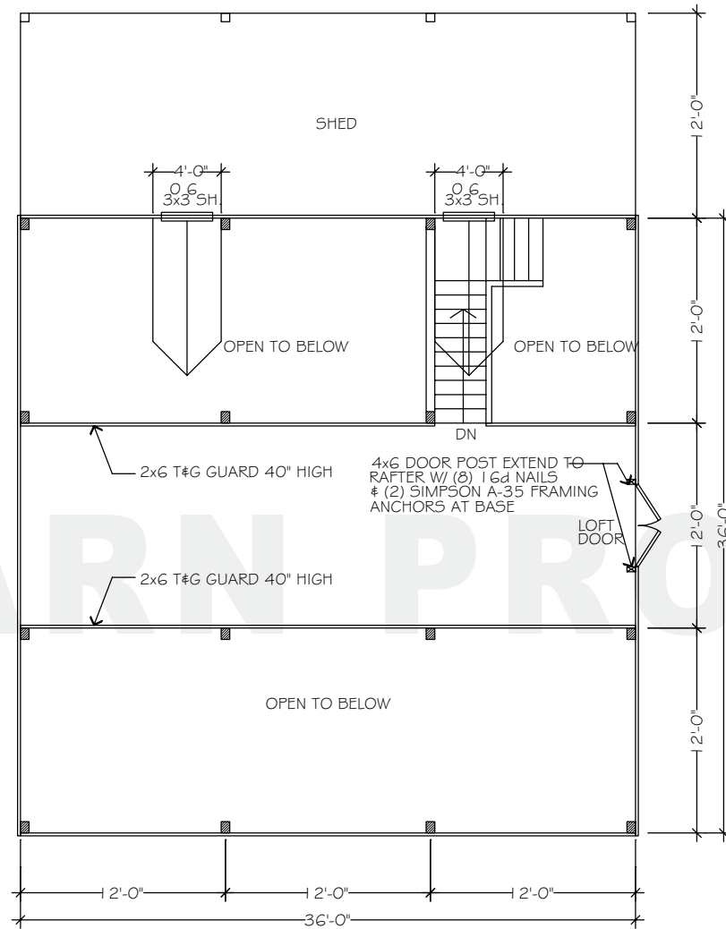
FLOORPLAN - UPPER
