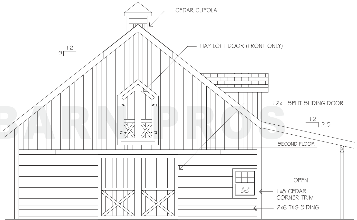
FRONT ELEVATION
