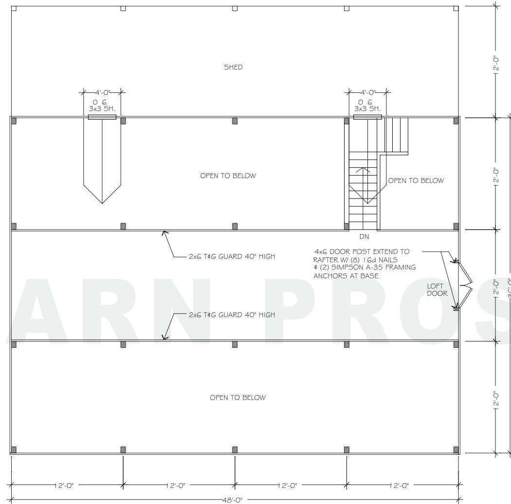
FLOORPLAN - UPPER
