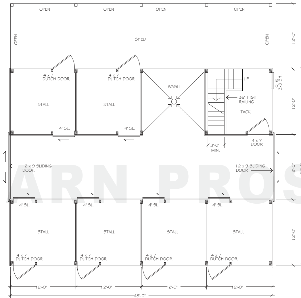
FLOORPLAN - LOWER
