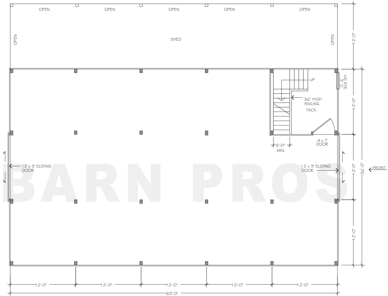
FLOORPLAN - LOWER
