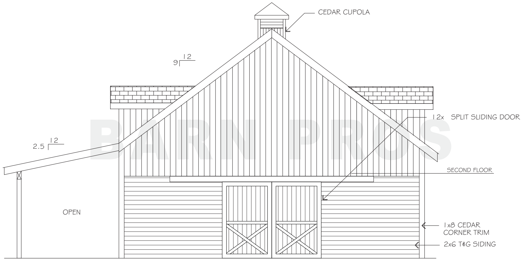
REAR ELEVATION
