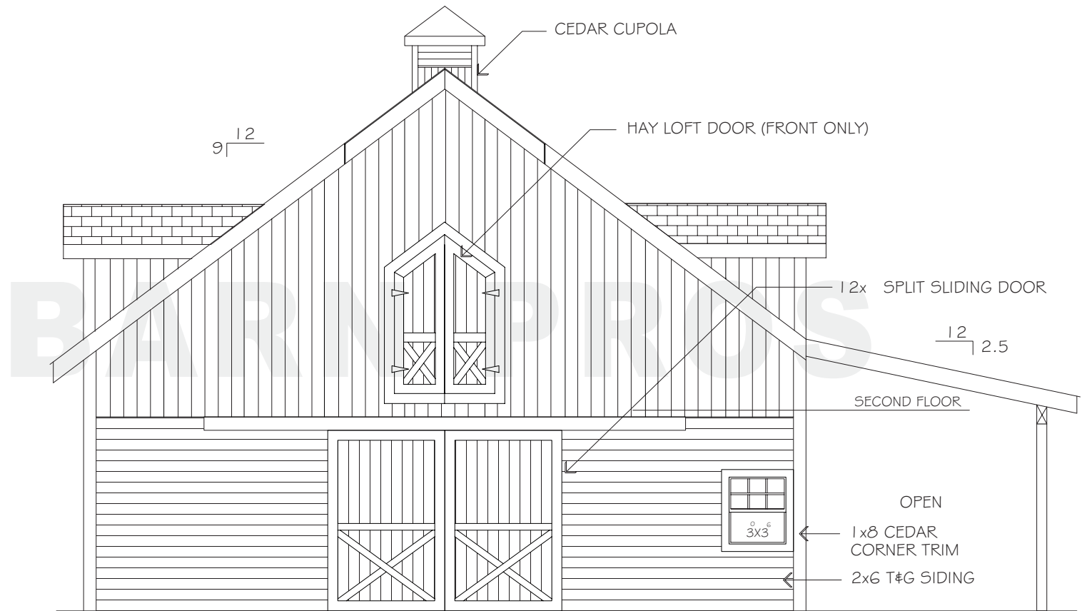
FRONT ELEVATION
