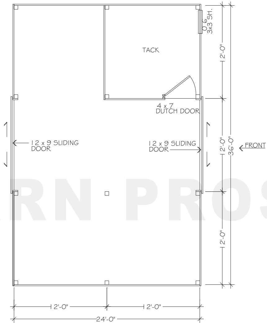
FLOORPLAN - LOWER
