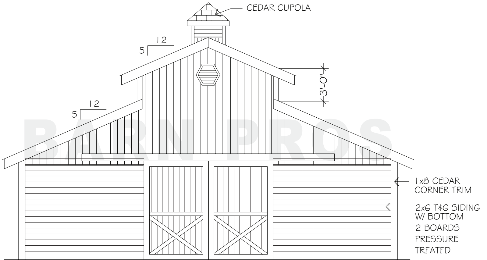
REAR ELEVATION
