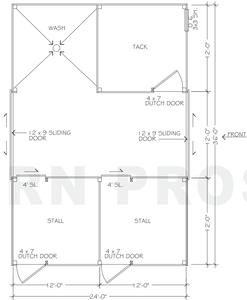
FLOORPLAN - LOWER
