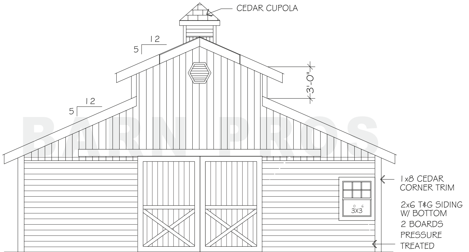
FRONT ELEVATION
