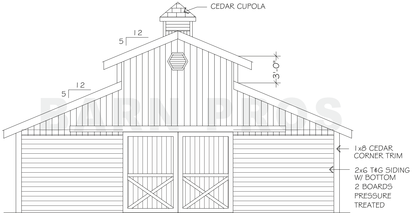
REAR ELEVATION
