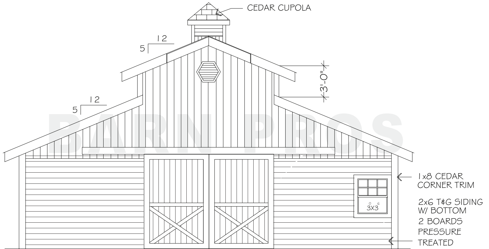
FRONT ELEVATION
