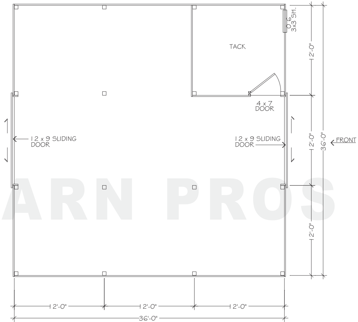
FLOORPLAN - LOWER
