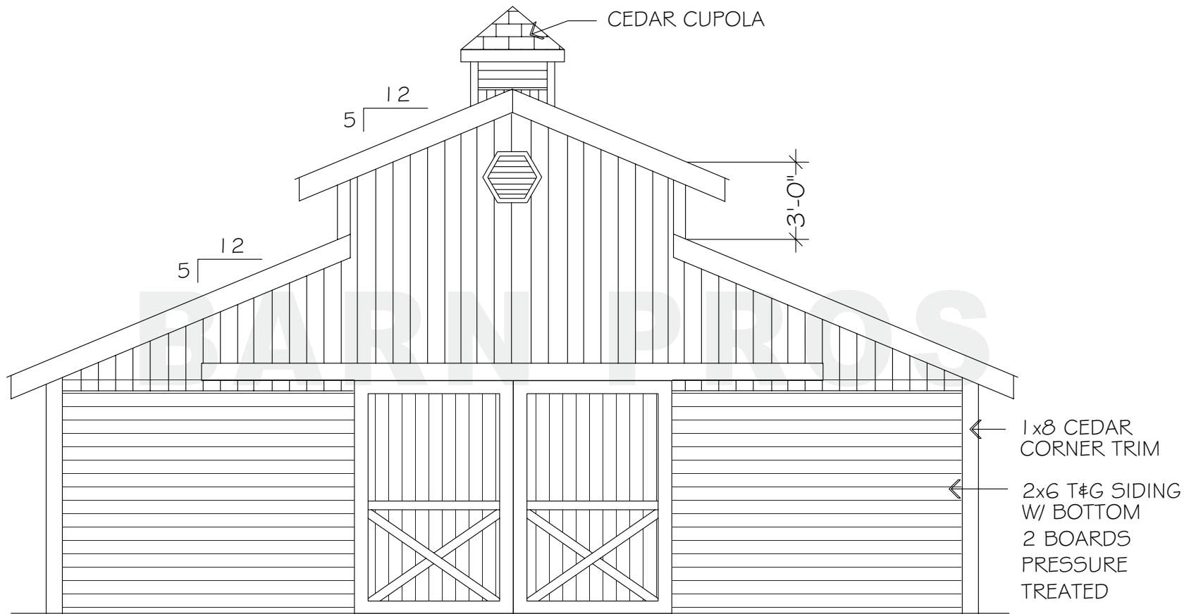
REAR ELEVATION
