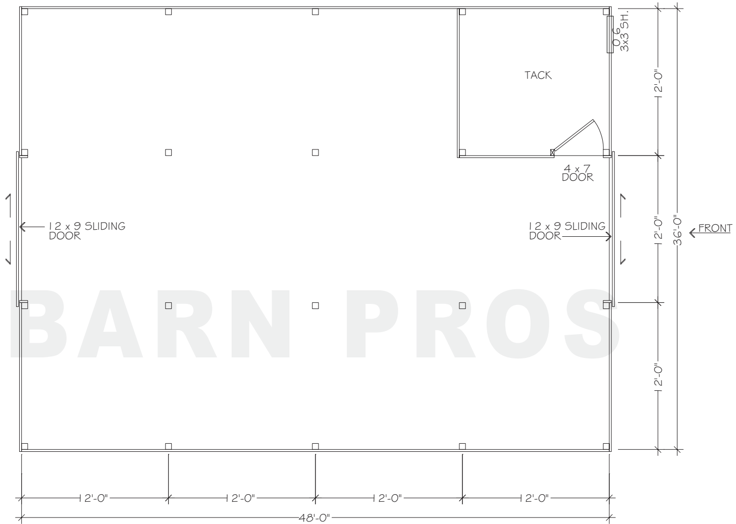
FLOORPLAN - LOWER
