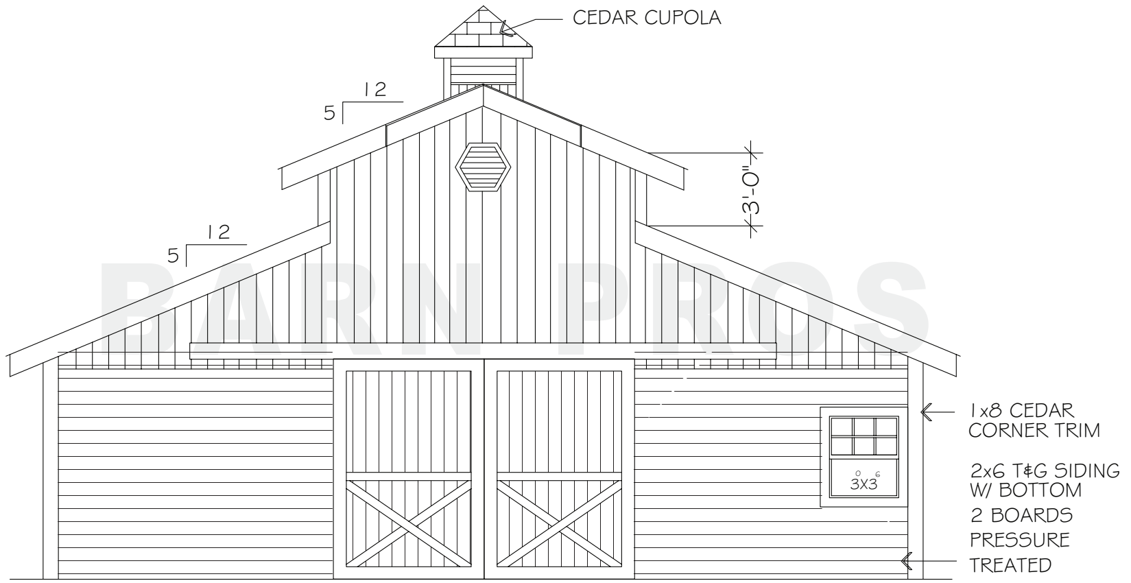
FRONT ELEVATION
