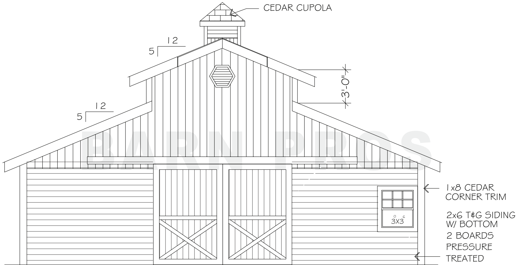
FRONT ELEVATION
