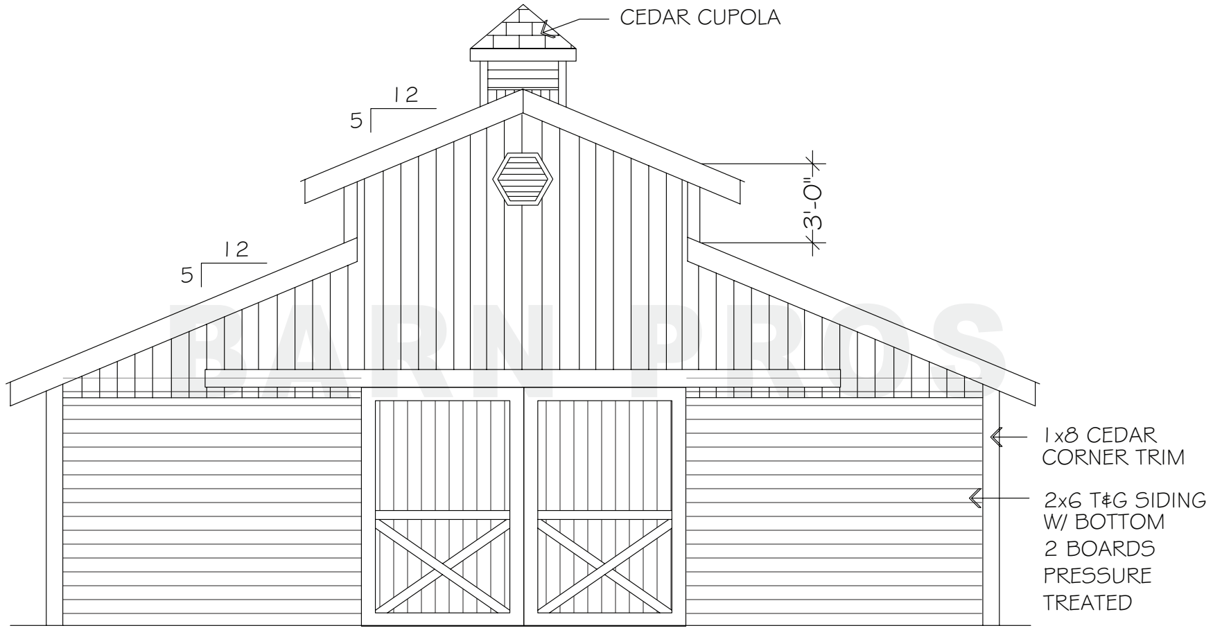
REAR ELEVATION
