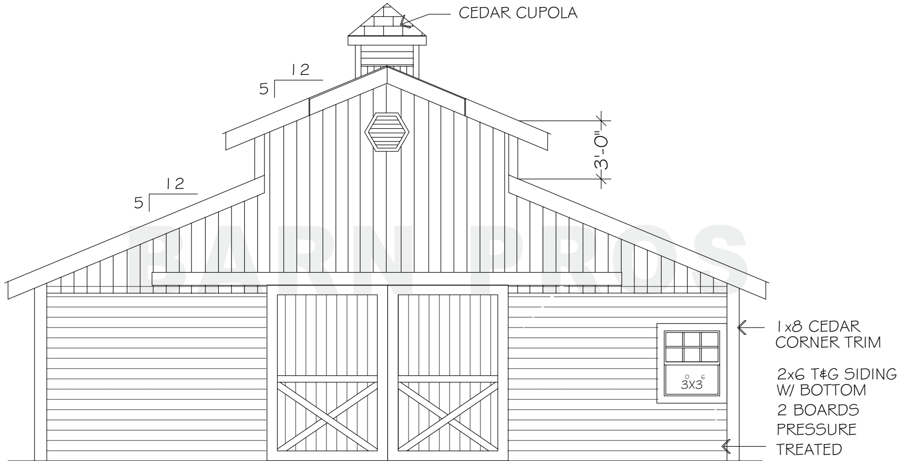
FRONT ELEVATION
