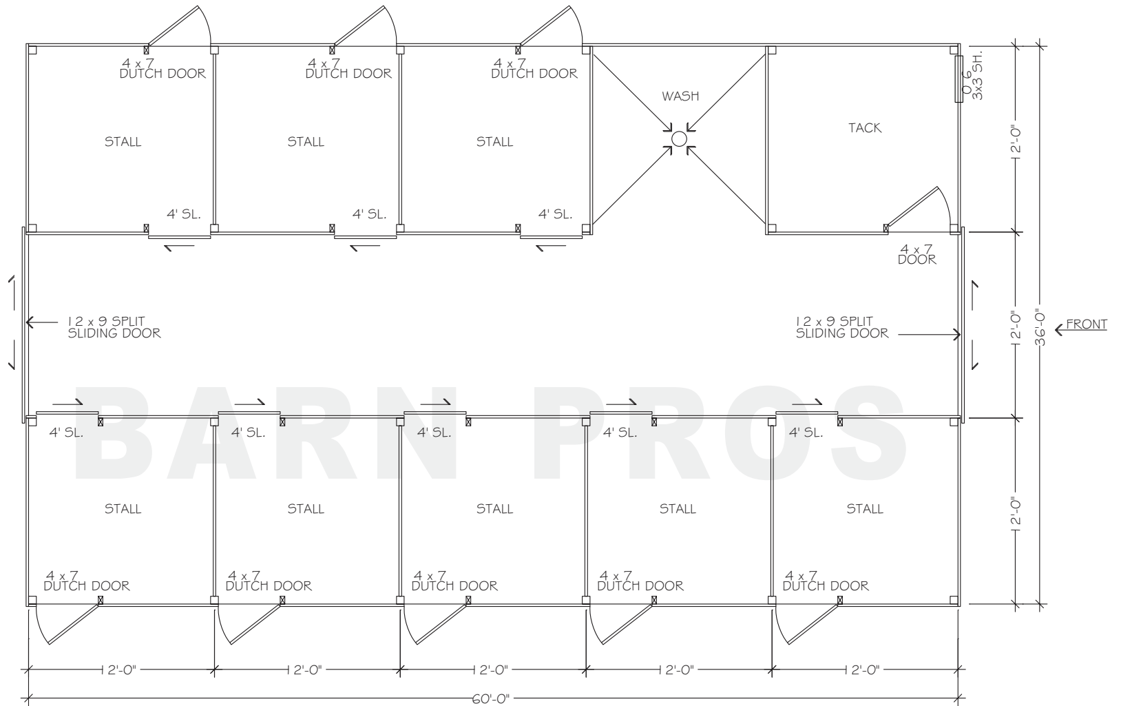
FLOORPLAN - LOWER
