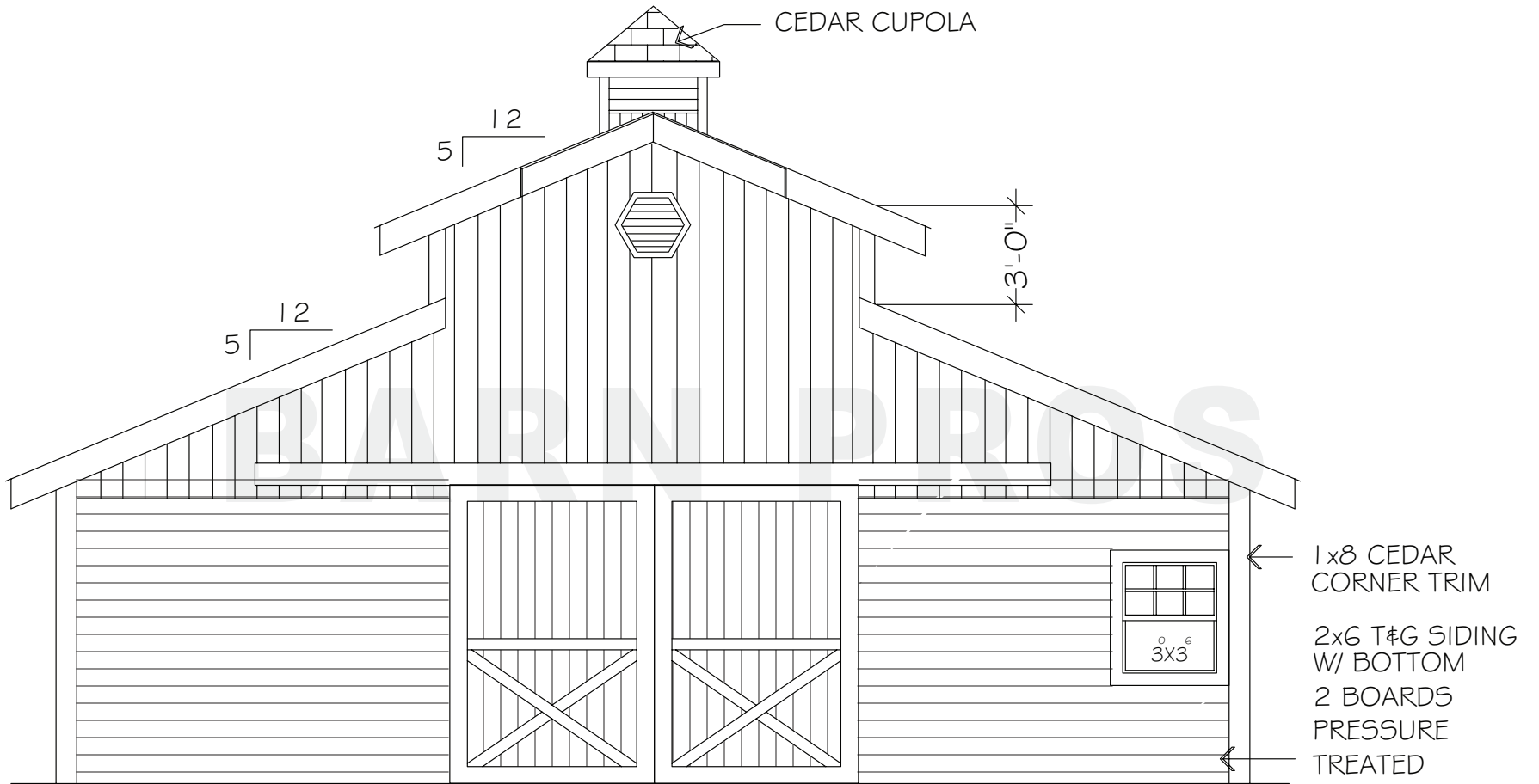
FRONT ELEVATION
