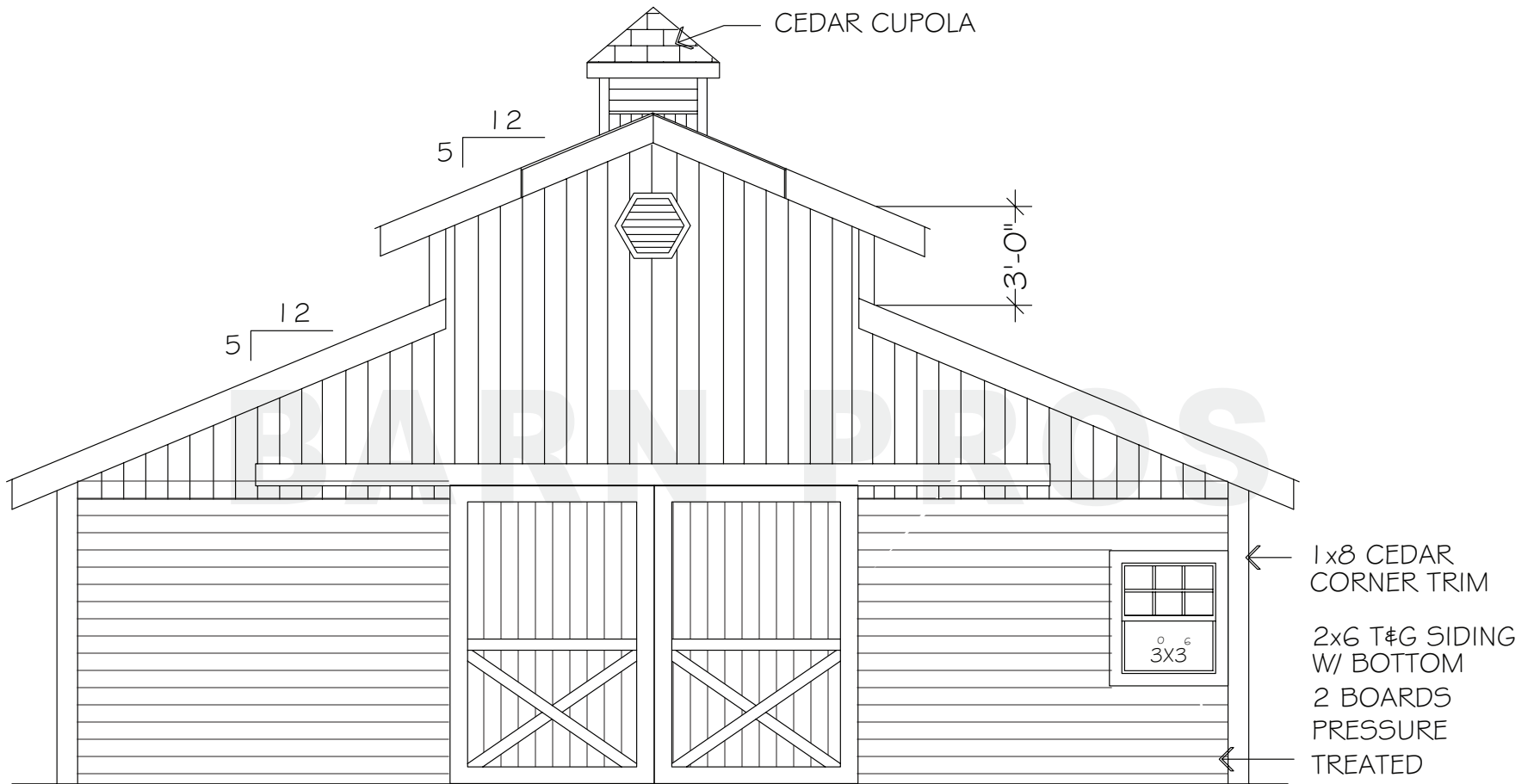
FRONT ELEVATION
