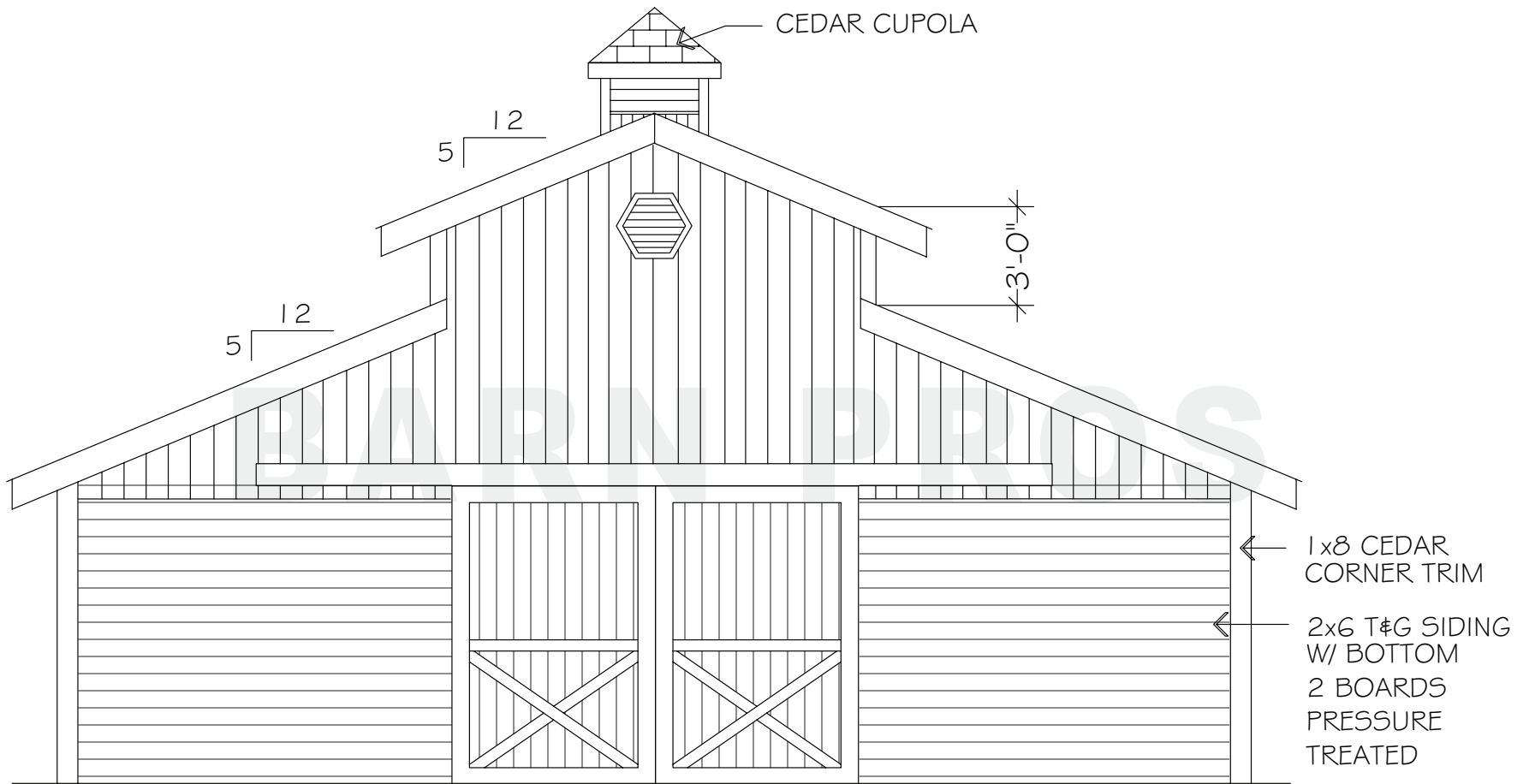
REAR ELEVATION
