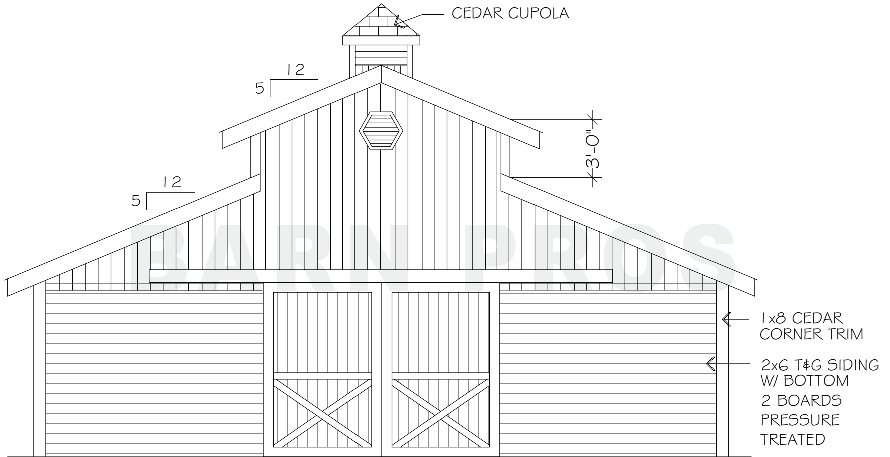
REAR ELEVATION
