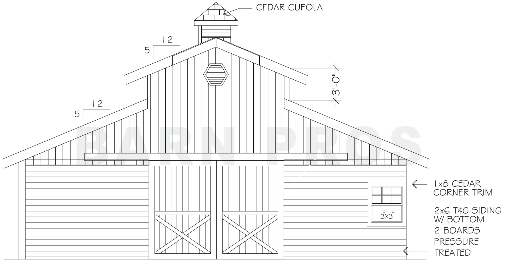
FRONT ELEVATION
