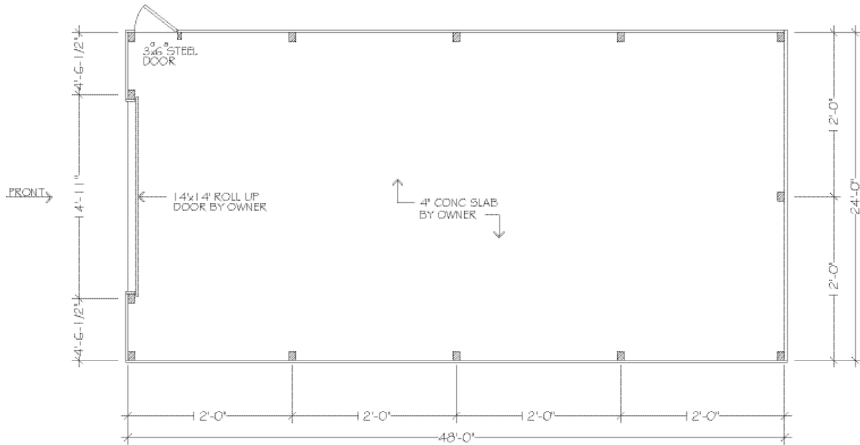
FLOORPLAN - LOWER
