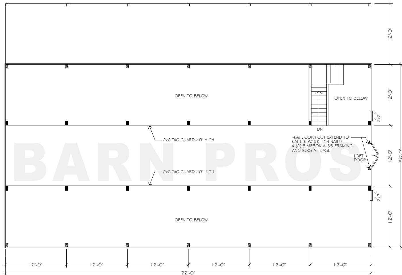
FLOORPLAN - UPPER
