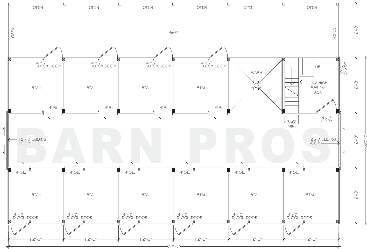
FLOORPLAN - LOWER
